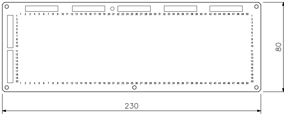
DB014 PCB
